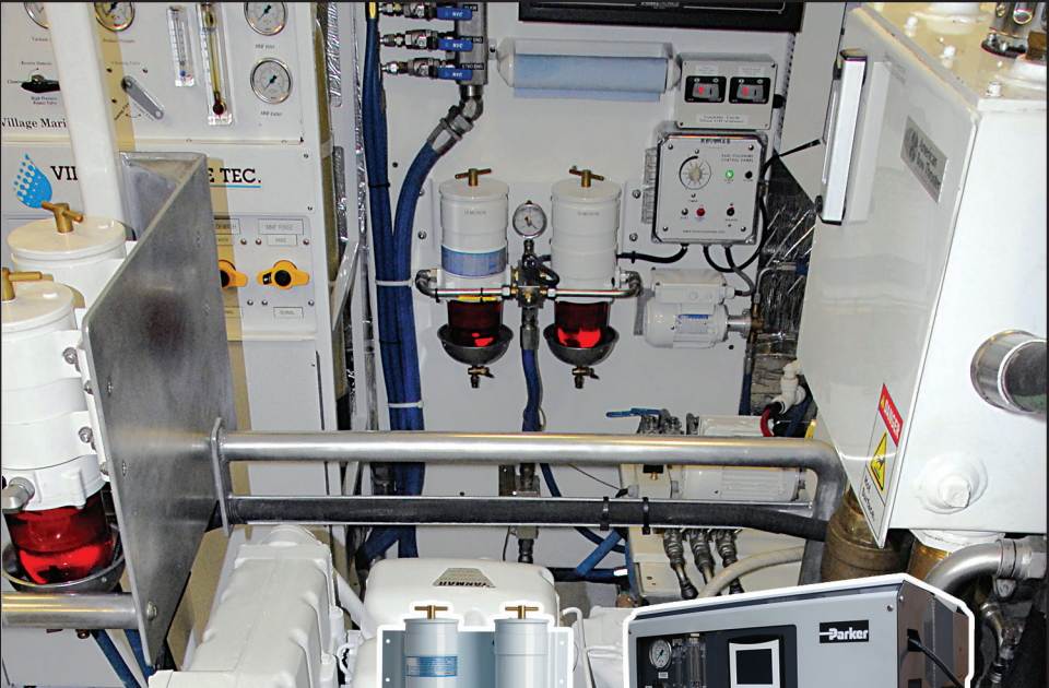
Racor Marine Turbine Series Fuel Filter/Water Separators
